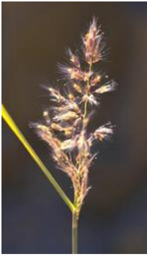
Tricholaena teneriffae
